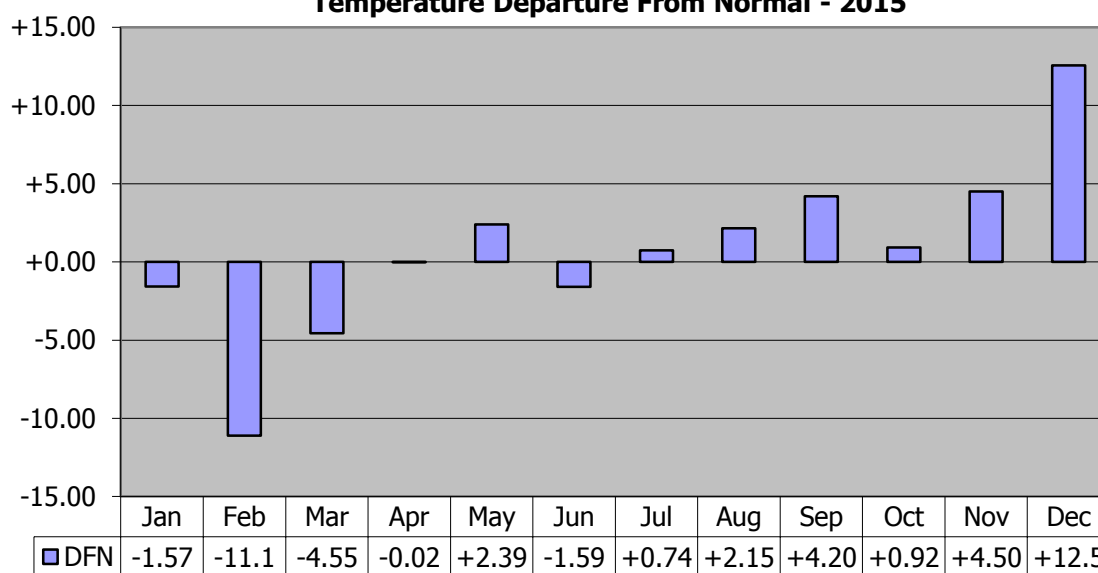
Temperature Departure From Normal - 2015
