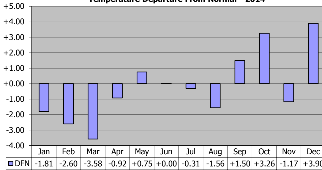
Temperature Departure From Normal - 2014
