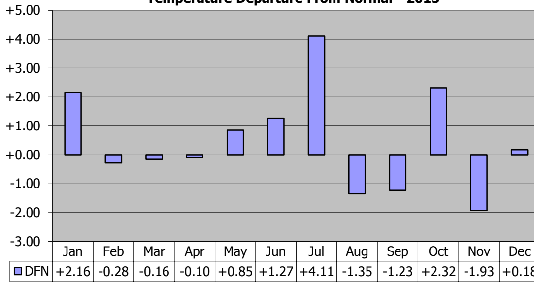
Temperature Departure From Normal - 2013
