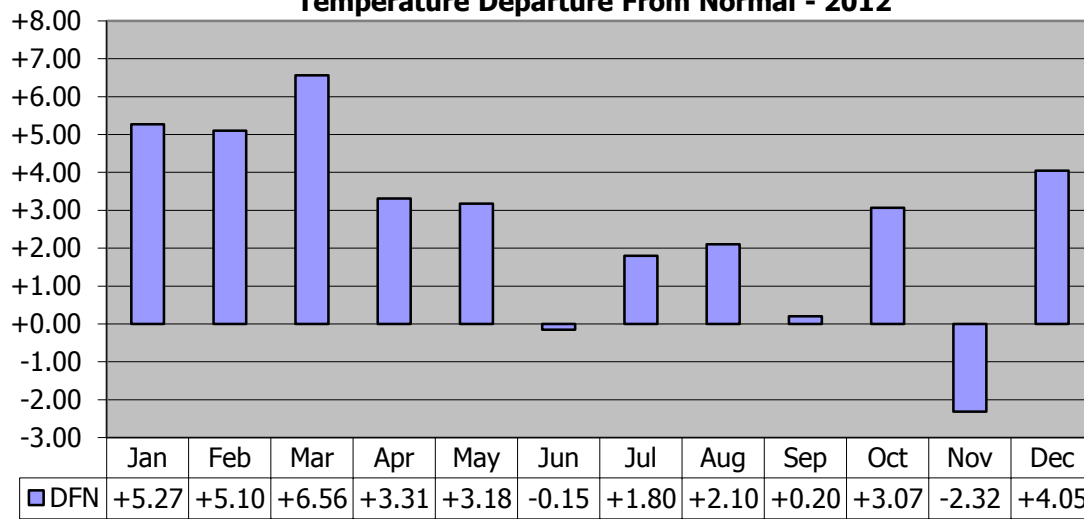
Temperature Departure From Normal - 2012
