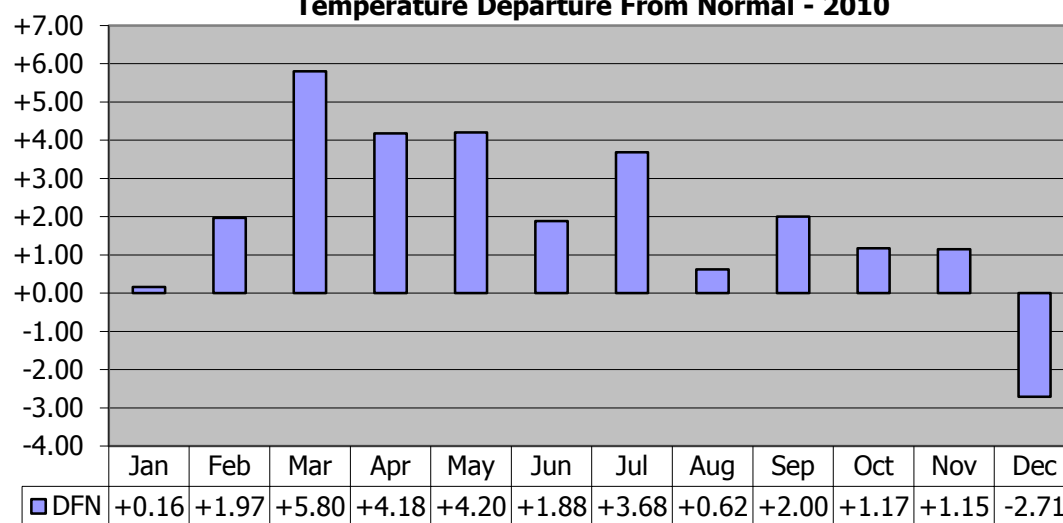
Temperature Departure From Normal - 2010
