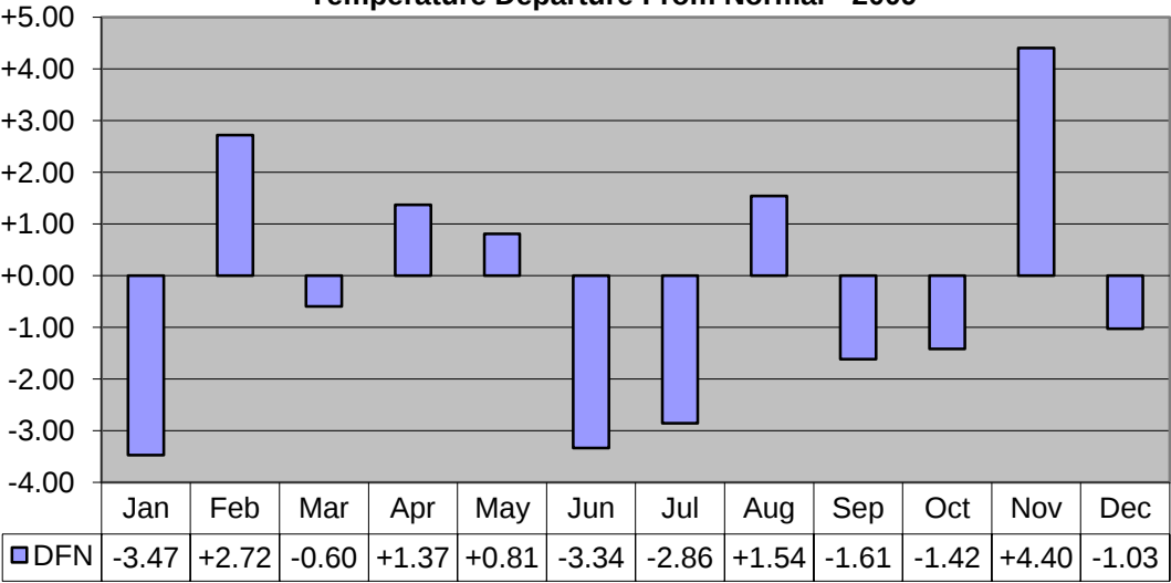
Temperature Departure From Normal - 2009
