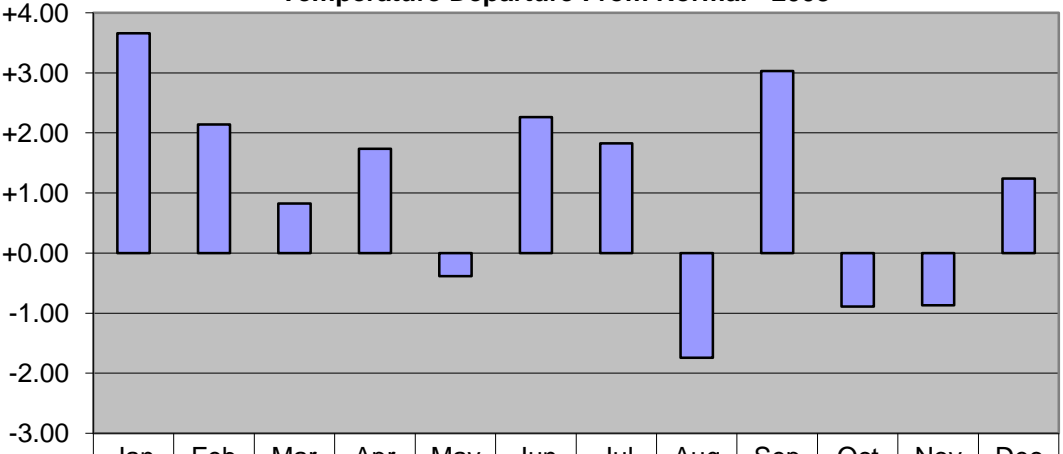
Temperature Departure From Normal - 2008
