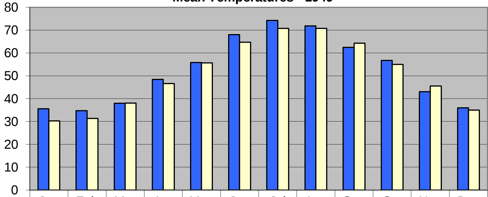
Mean Temperatures - 1949
