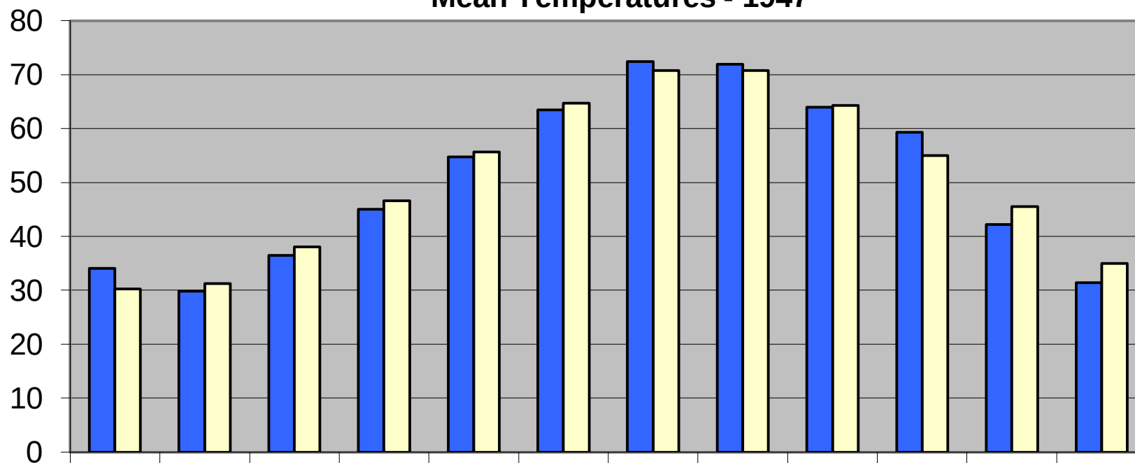
Mean Temperatures - 1947
