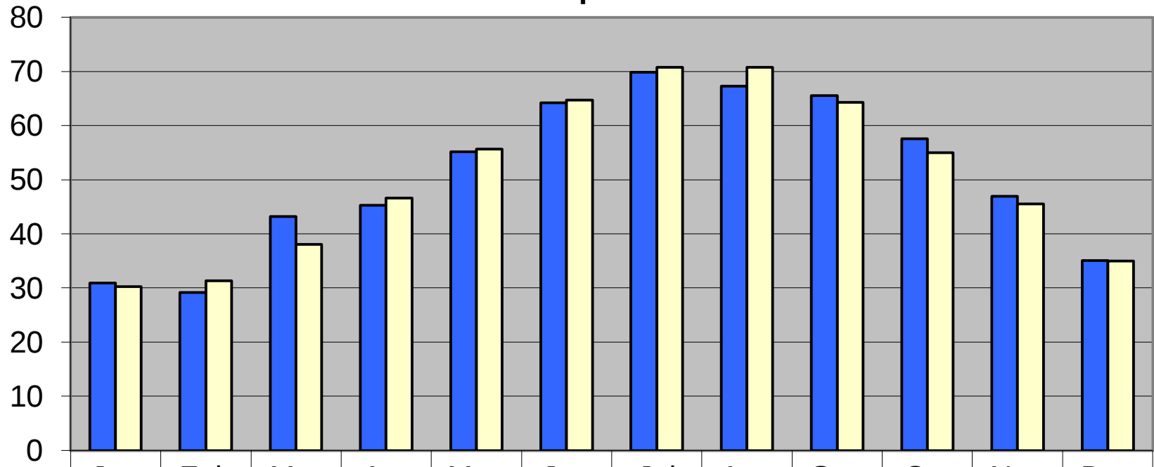
Mean Temperatures - 1946
