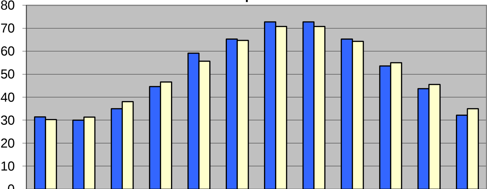
Mean Temperatures - 1944
