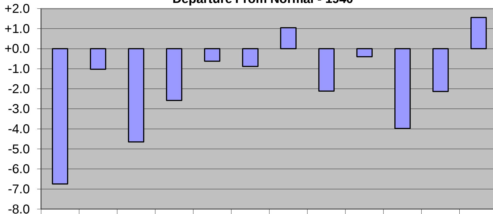
Departure From Normal - 1940
