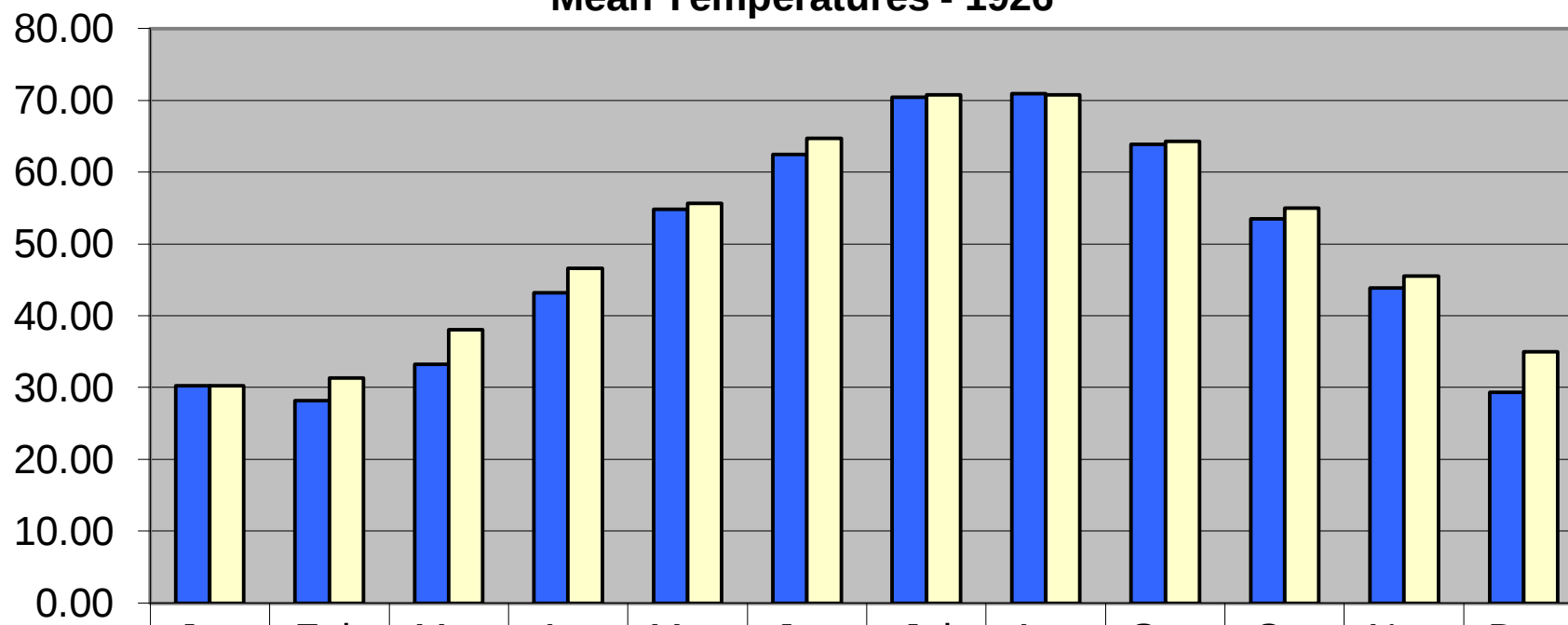
Mean Temperatures - 1926
