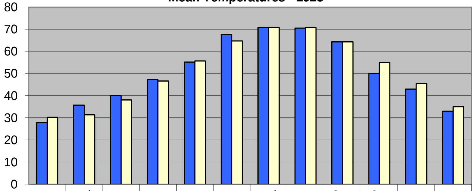
Mean Temperatures - 1925
