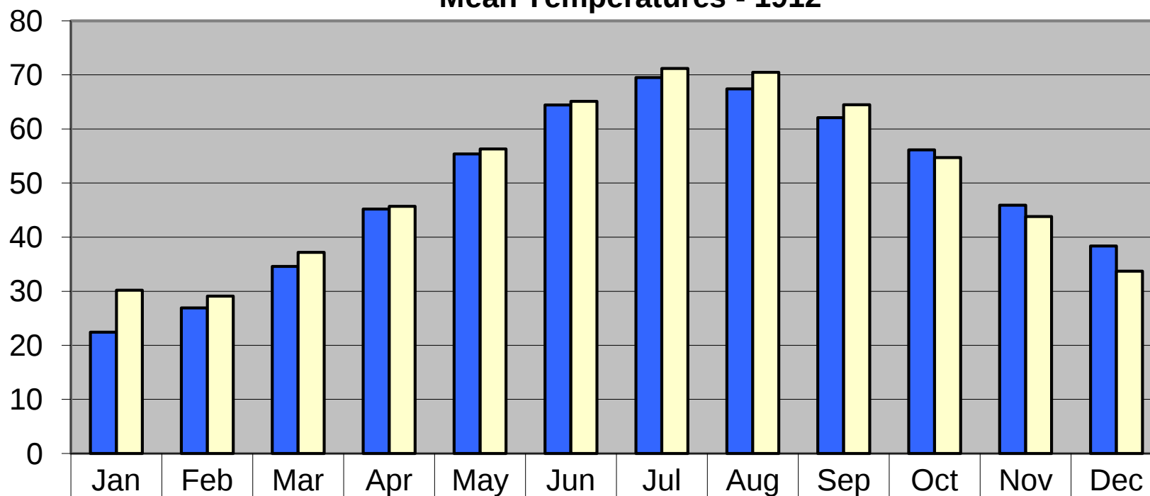
Mean Temperatures - 1912
