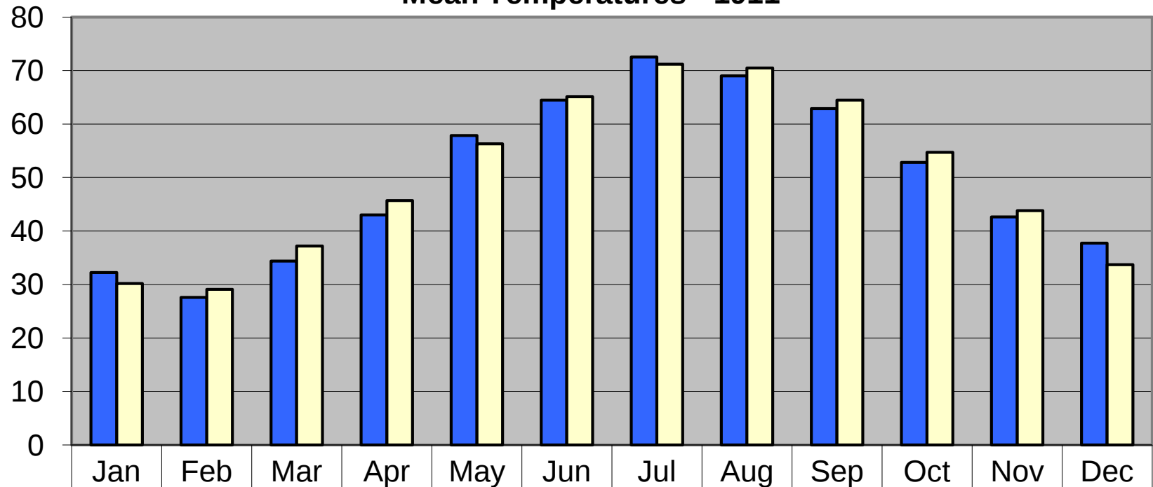
Mean Temperatures - 1911
