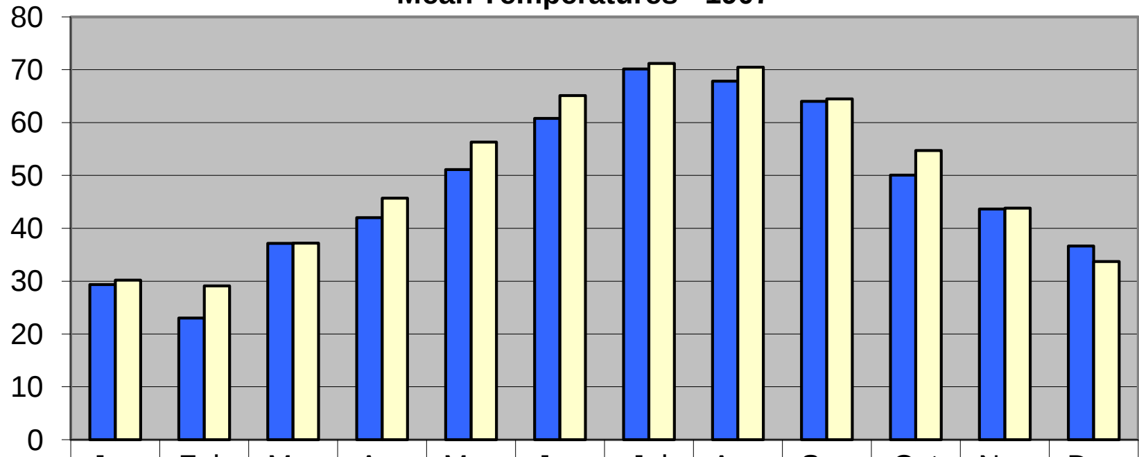
Mean Temperatures - 1907
