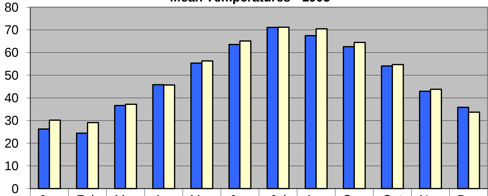
Mean Temperatures - 1905
