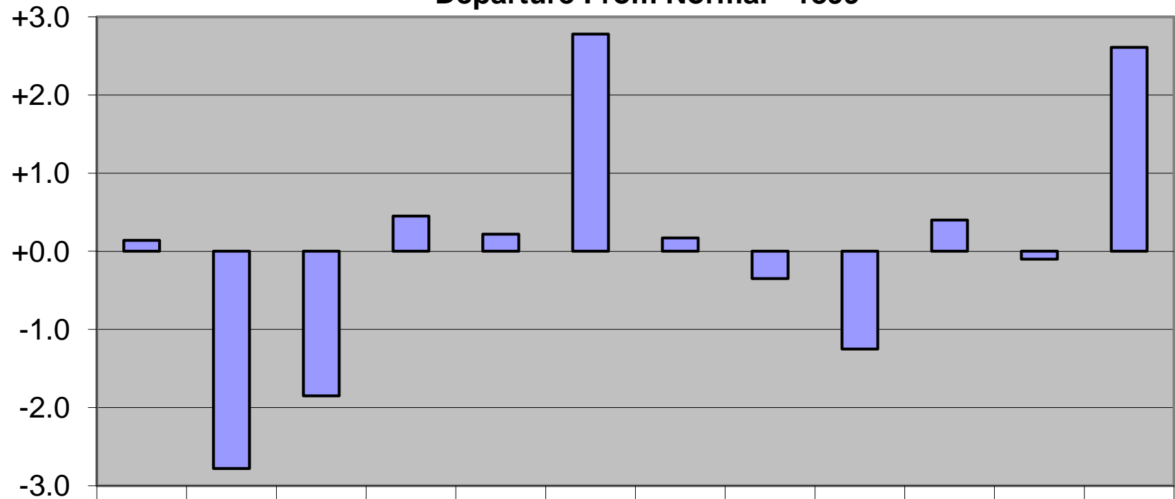
Departure From Normal - 1899
