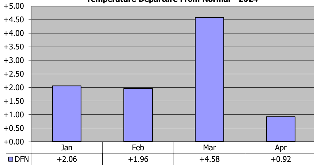
Temperature Departure From Normal - 2024
