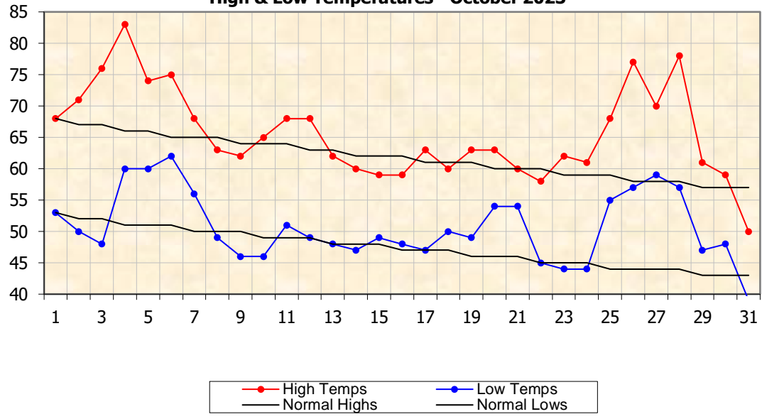
High & Low Temperatures - October 2023
