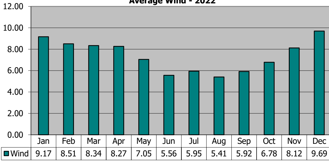
Average Wind - 2022
