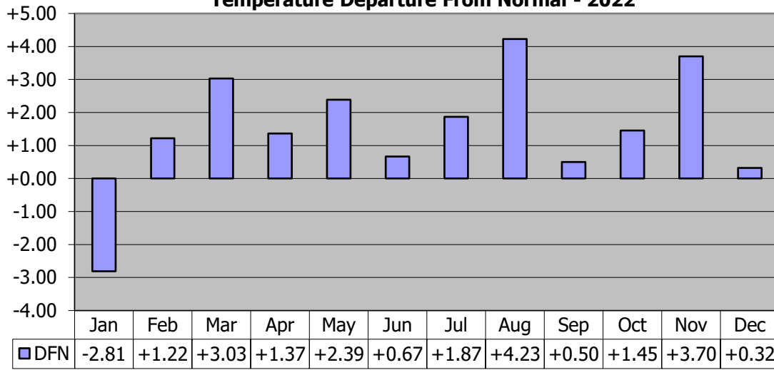
Temperature Departure From Normal - 2022
