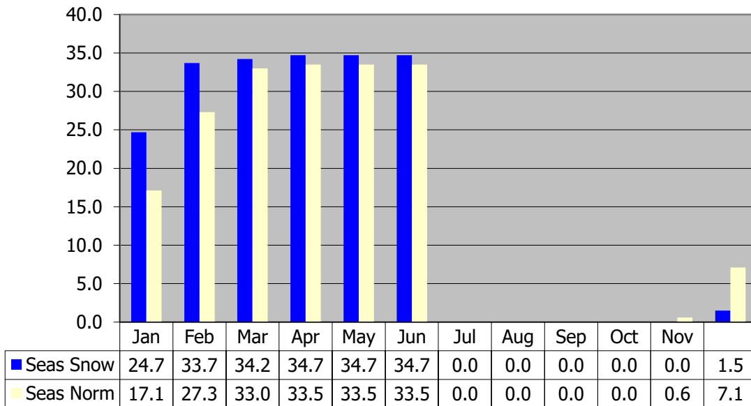
Season Snow - 2021-2022
