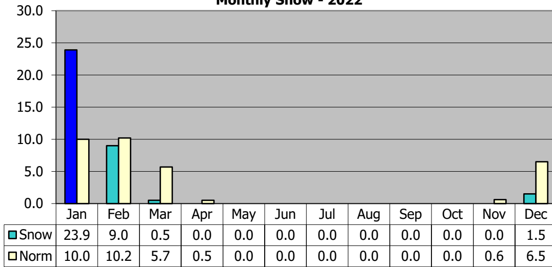
Monthly Snow - 2022
