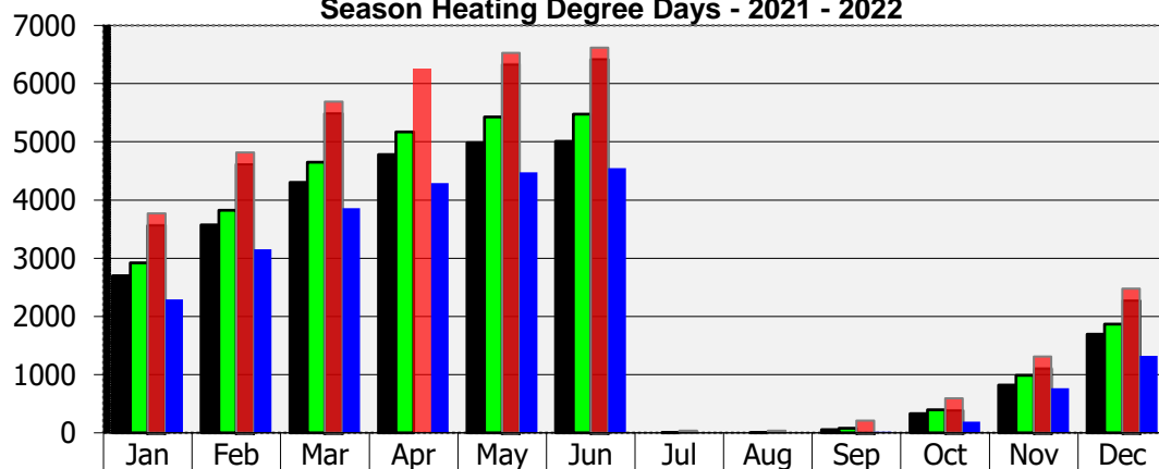
Season Heating Degree Days - 2021 - 2022
