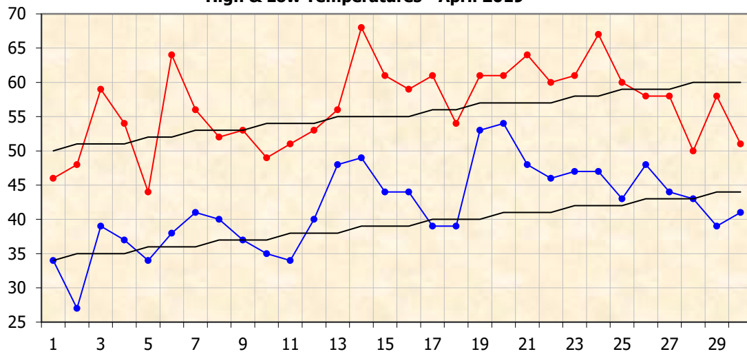
High & Low Temperatures - April 2019
