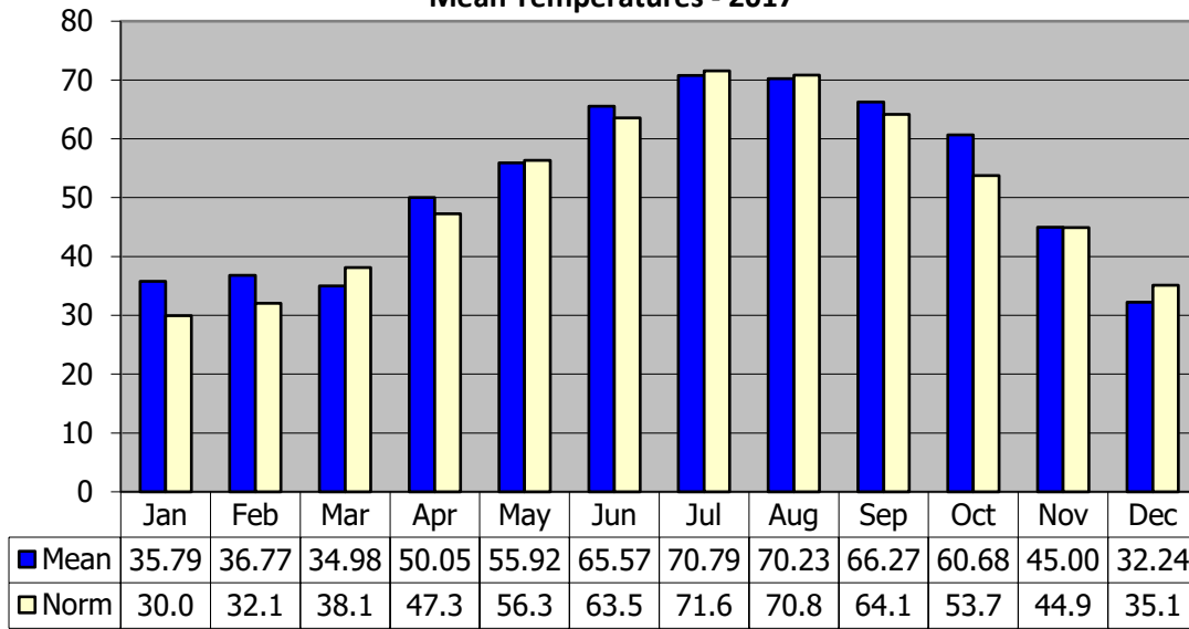
Mean Temperatures - 2017
