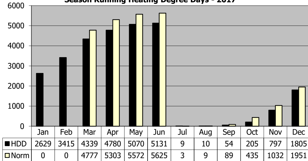
Season Running Heating Degree Days - 2017
