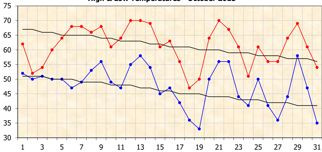
High & Low Temperatures - October 2015
