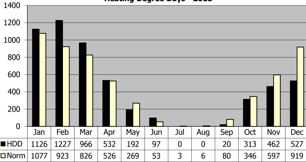
Heating Degree Days - 2015
