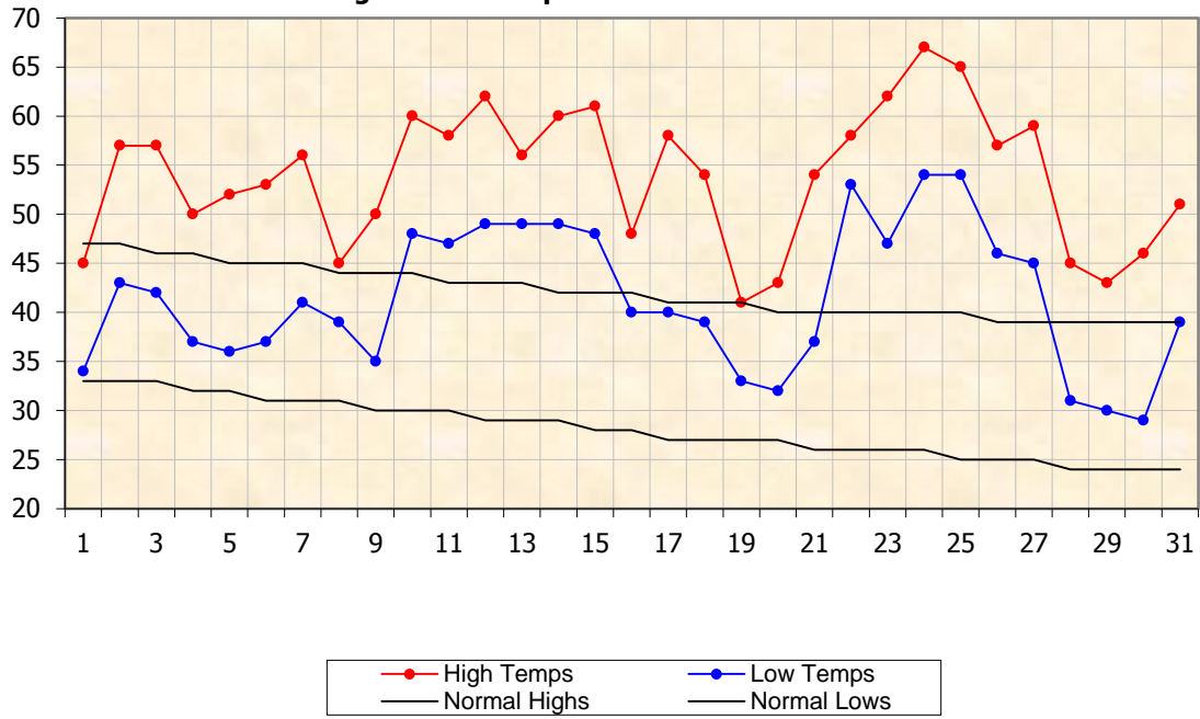
High & Low Temperatures - December 2015
