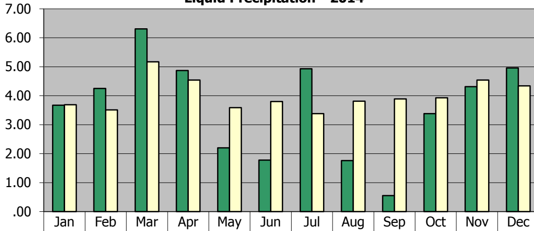
Liquid Precipitation - 2014
