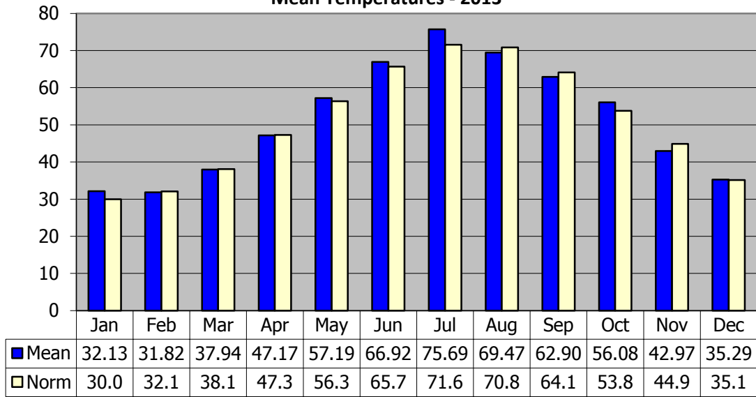
Mean Temperatures - 2013
