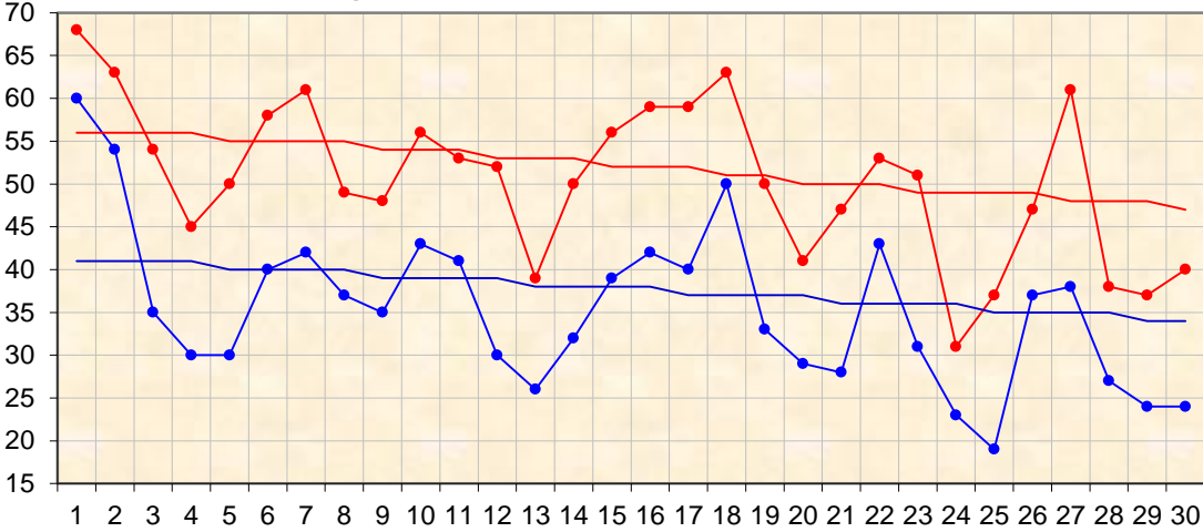
High & Low Temperatures - November 2013
