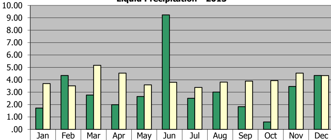
Liquid Precipitation - 2013
