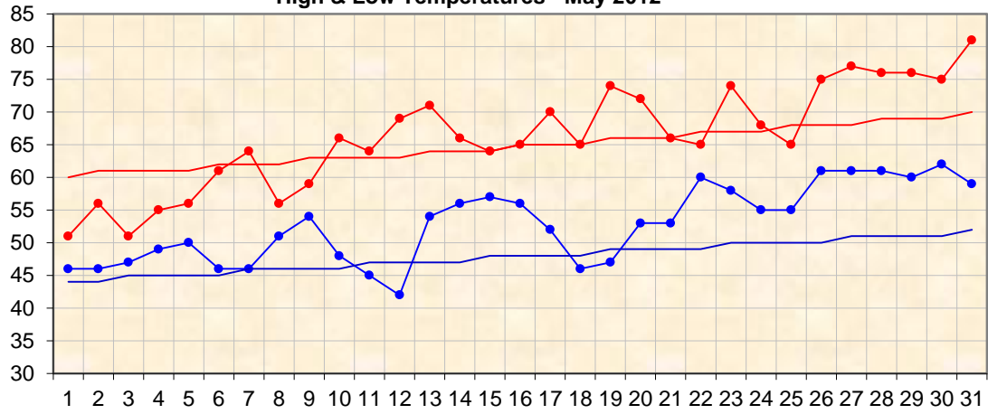
High & Low Temperatures - May 2012
