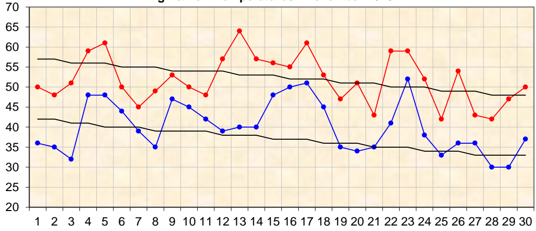
High & Low Temperatures - November 2010
