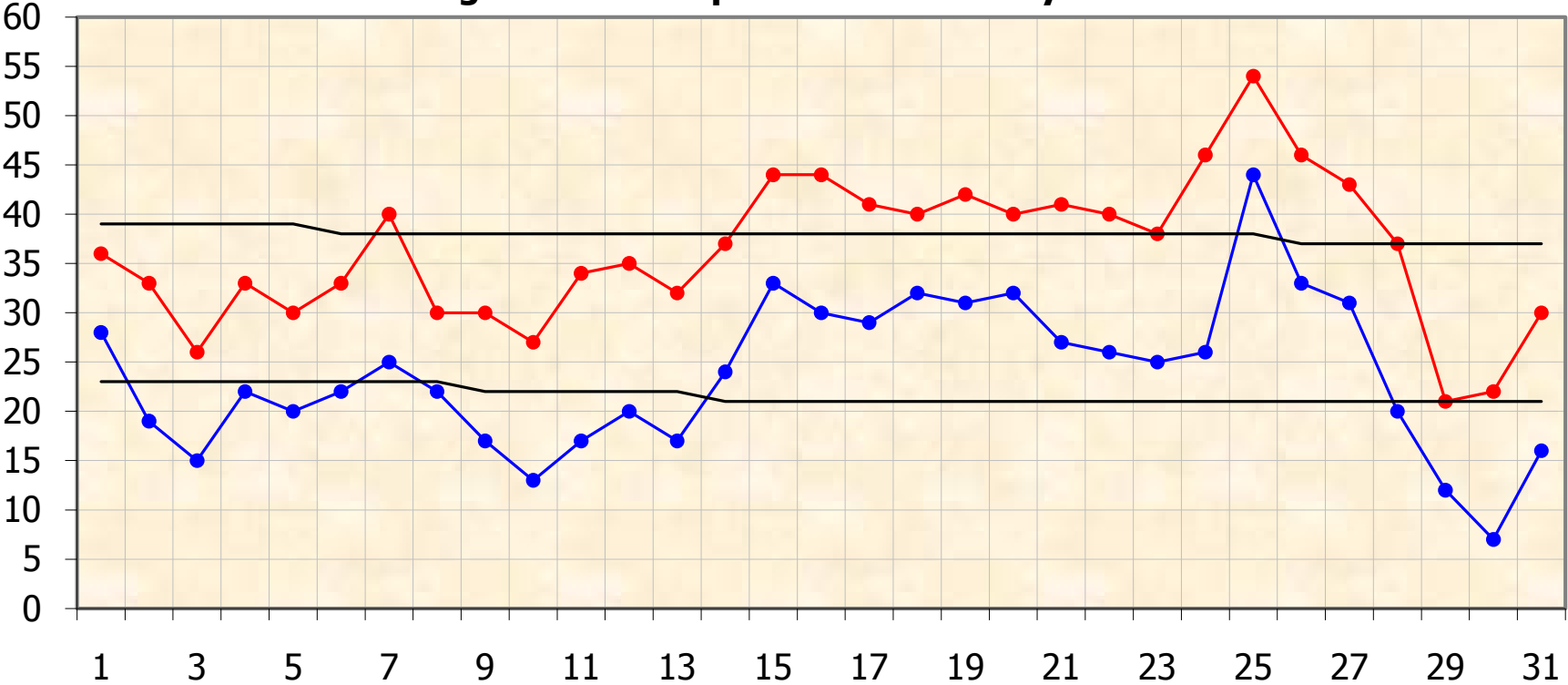
High & Low Temperatures - January 2010
