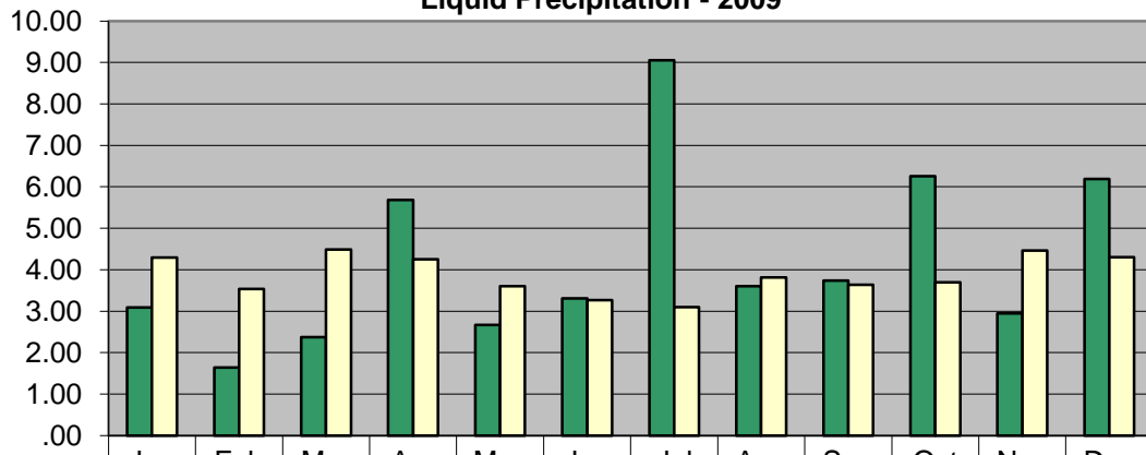
Liquid Precipitation - 2009
