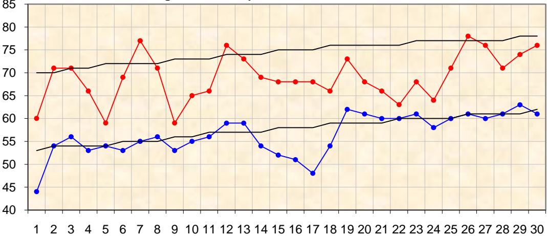
High & Low Temperatures - June 2009
