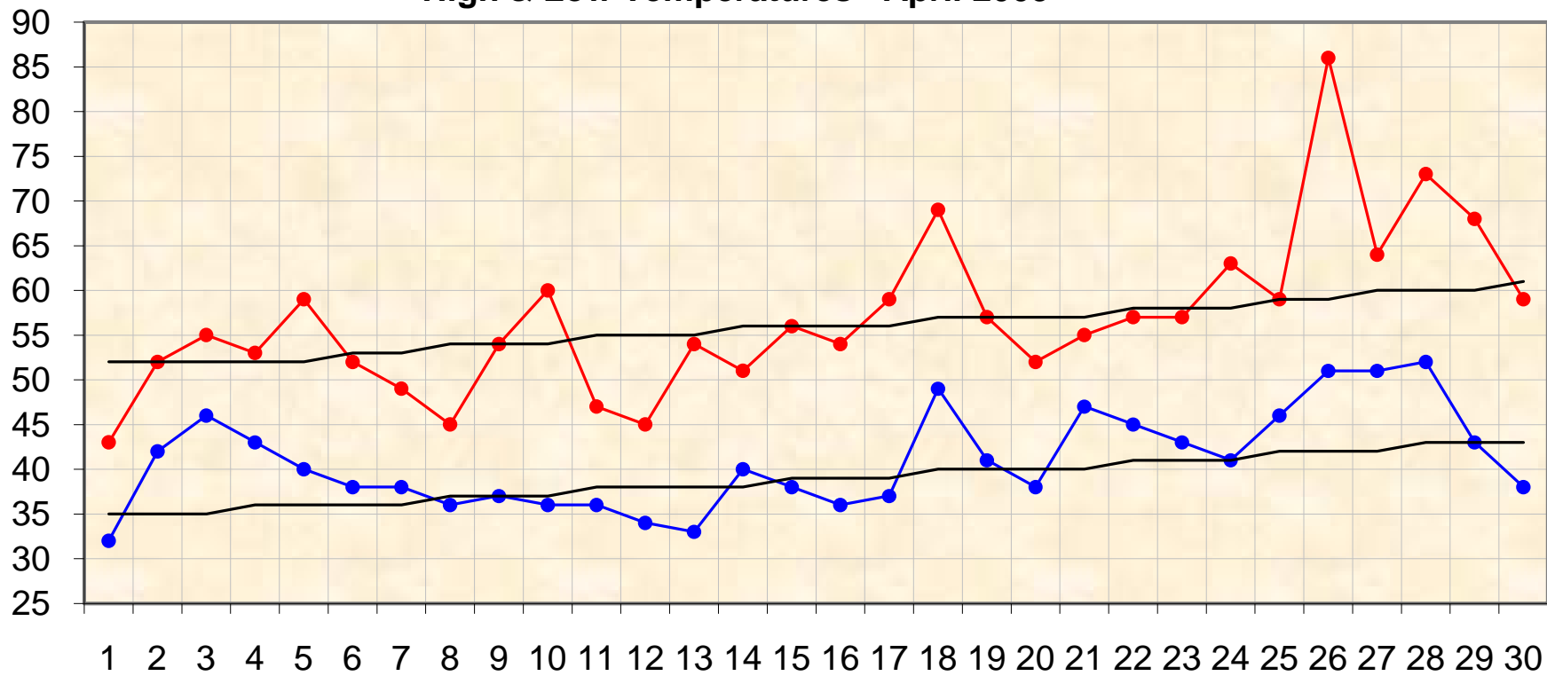
High & Low Temperatures - April 2009
