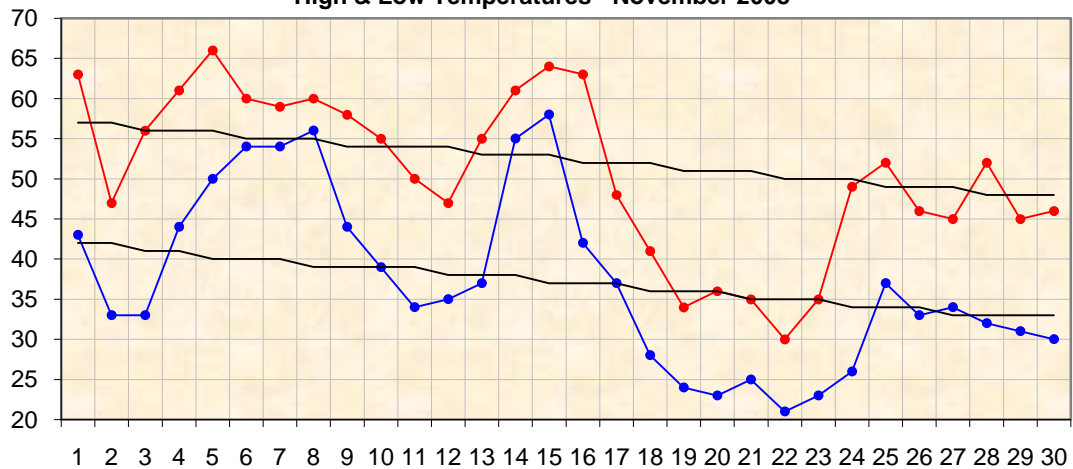
High & Low Temperatures - November 2008
