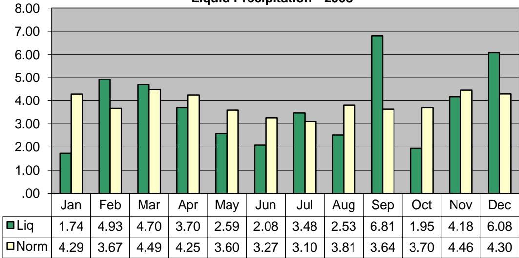
Liquid Precipitation - 2008
