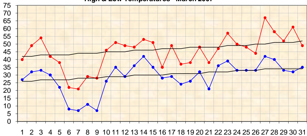
High & Low Temperatures - March 2007
