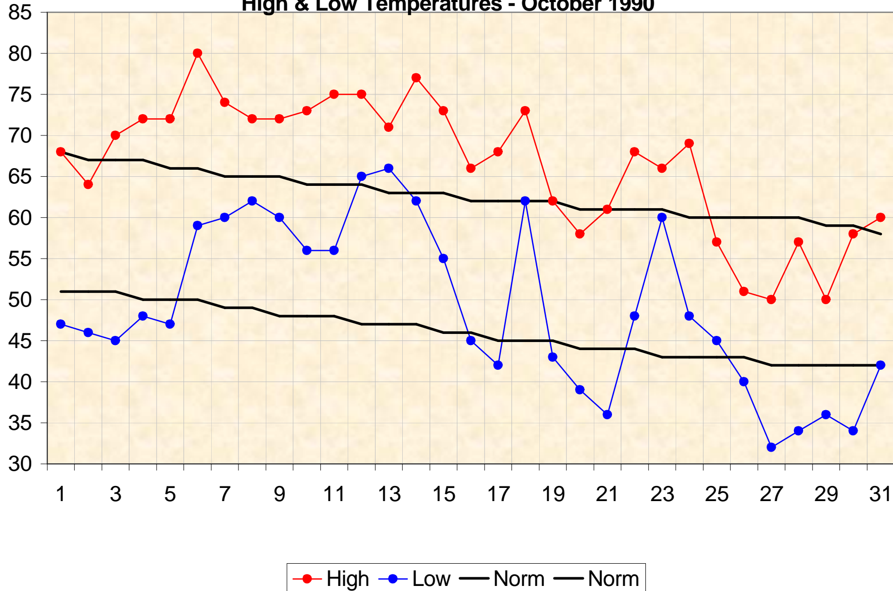
High & Low Temperatures - October 1990
