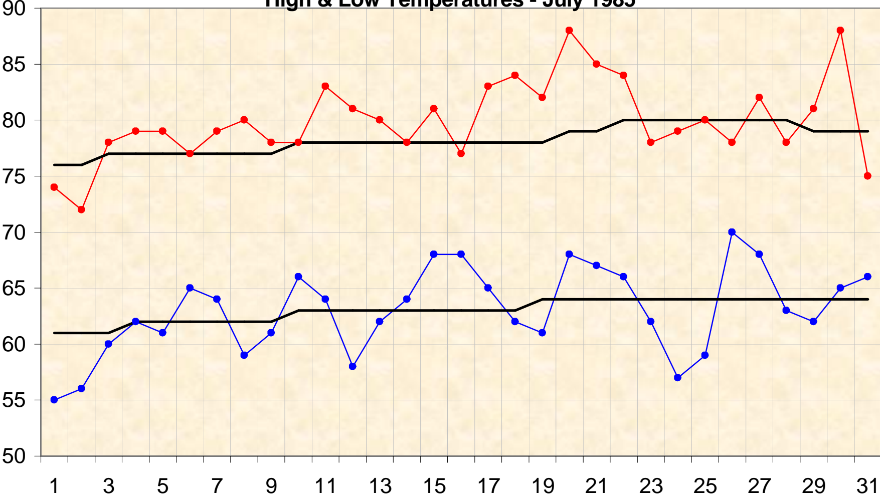
High & Low Temperatures - July 1985
