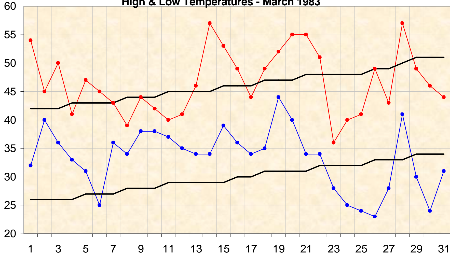
High & Low Temperatures - March 1983
