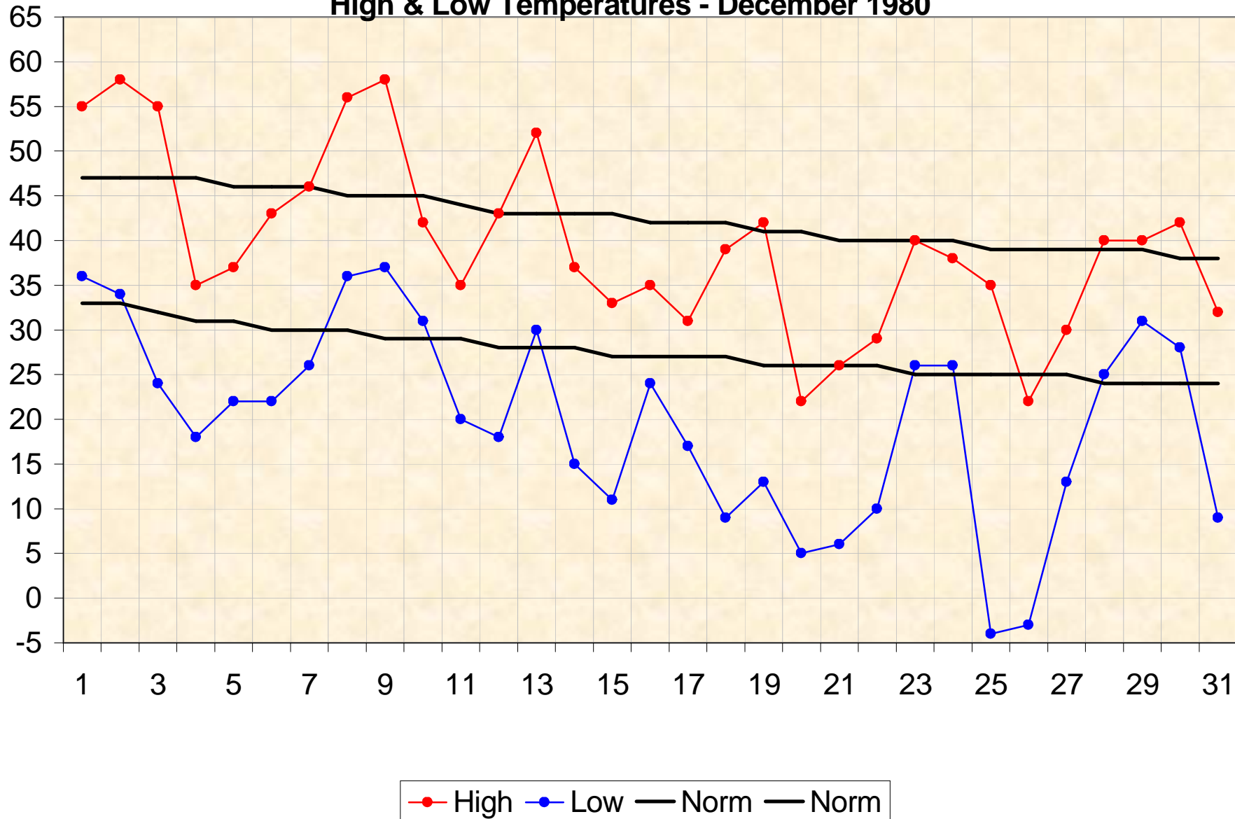
High & Low Temperatures - December 1980
