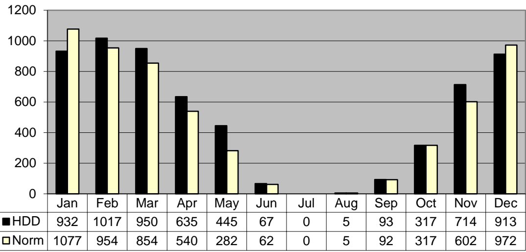
Heating Degree Days - 1967
