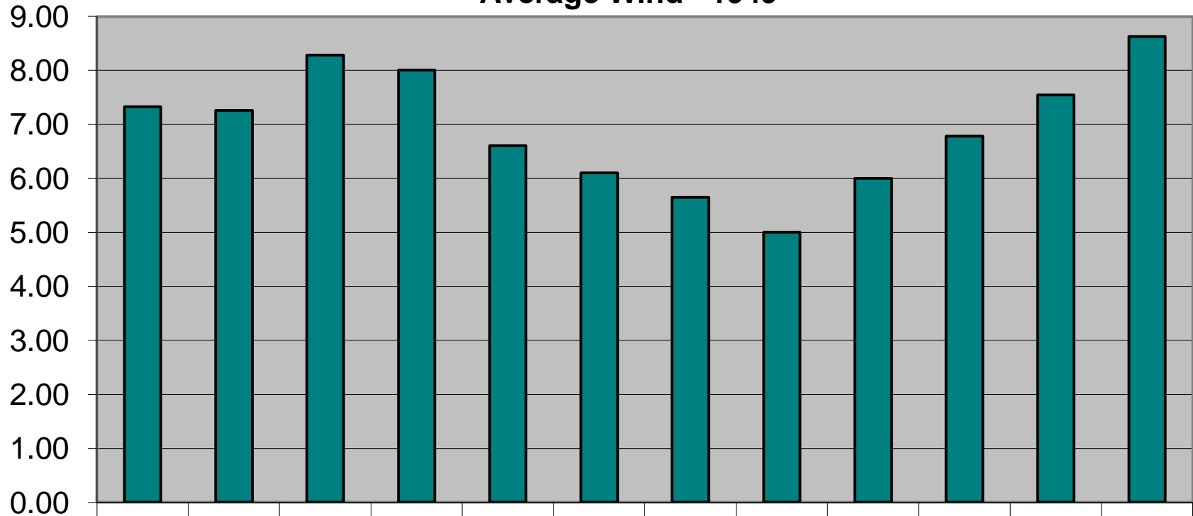
Average Wind - 1949
